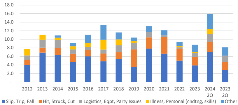
Climbing Incident Category Rate Trends
